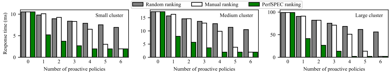
Fig. 14. Impact of ranking on average response time of policies ( Network profile)
